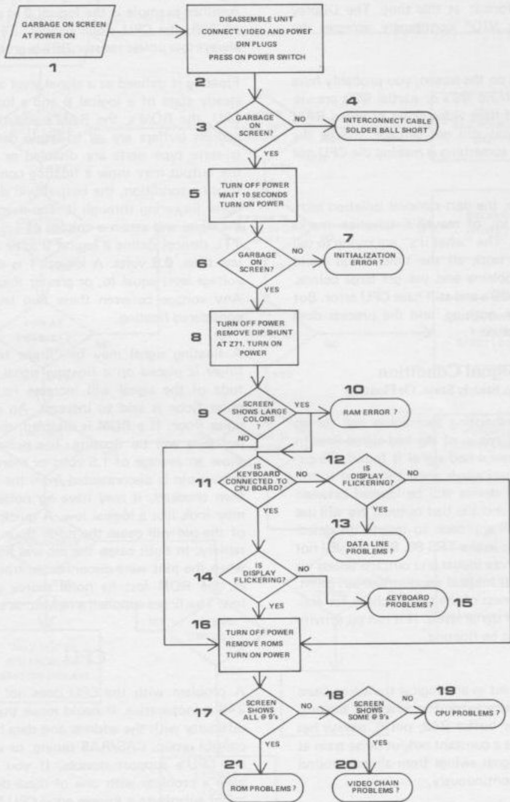
FIGURE 16. Section Isolation Flowchart
