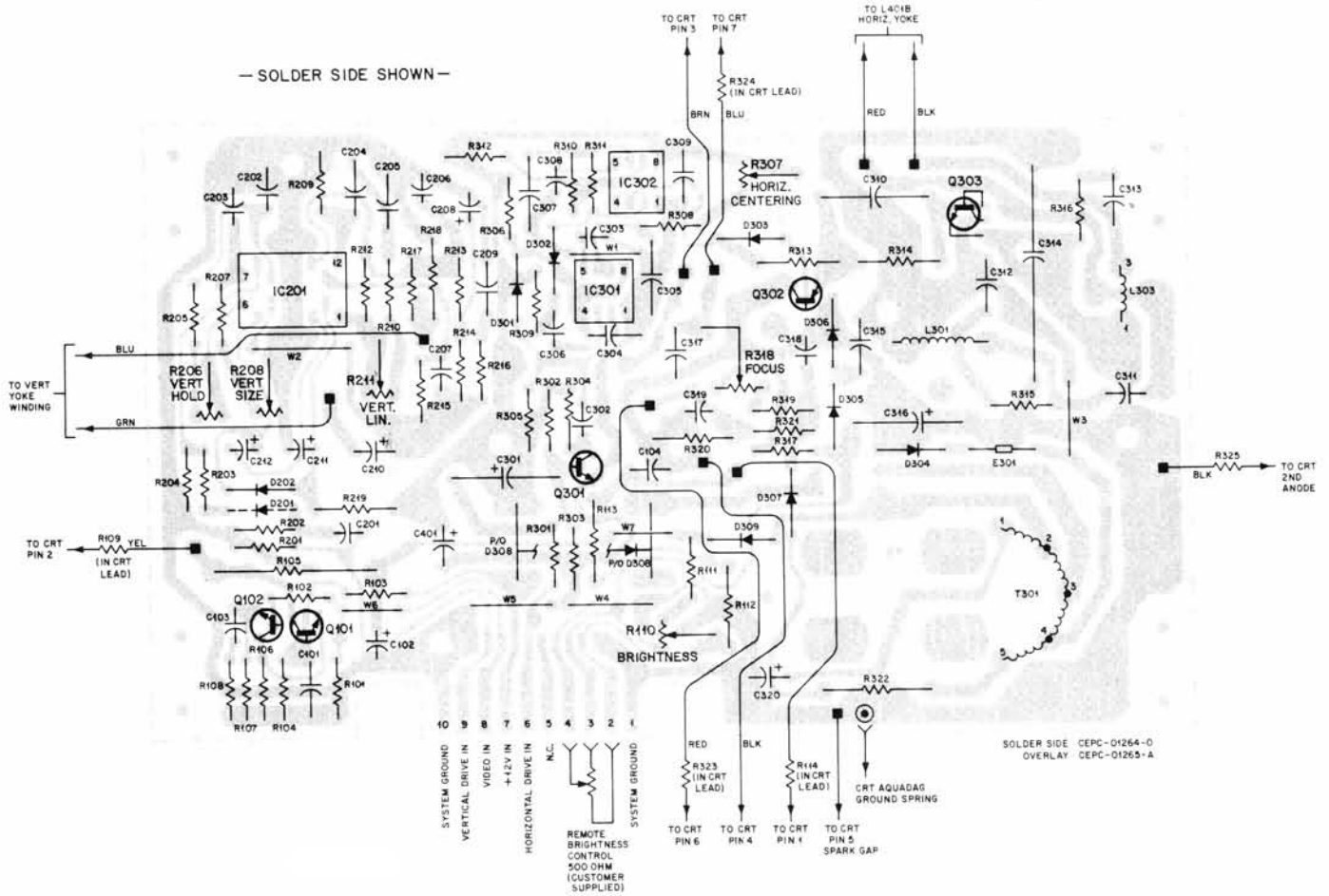
Model MD3570-4/MD3970-4 Series CRT Display Monitor Circuit Card Detail, Solder Side (Early Version)
