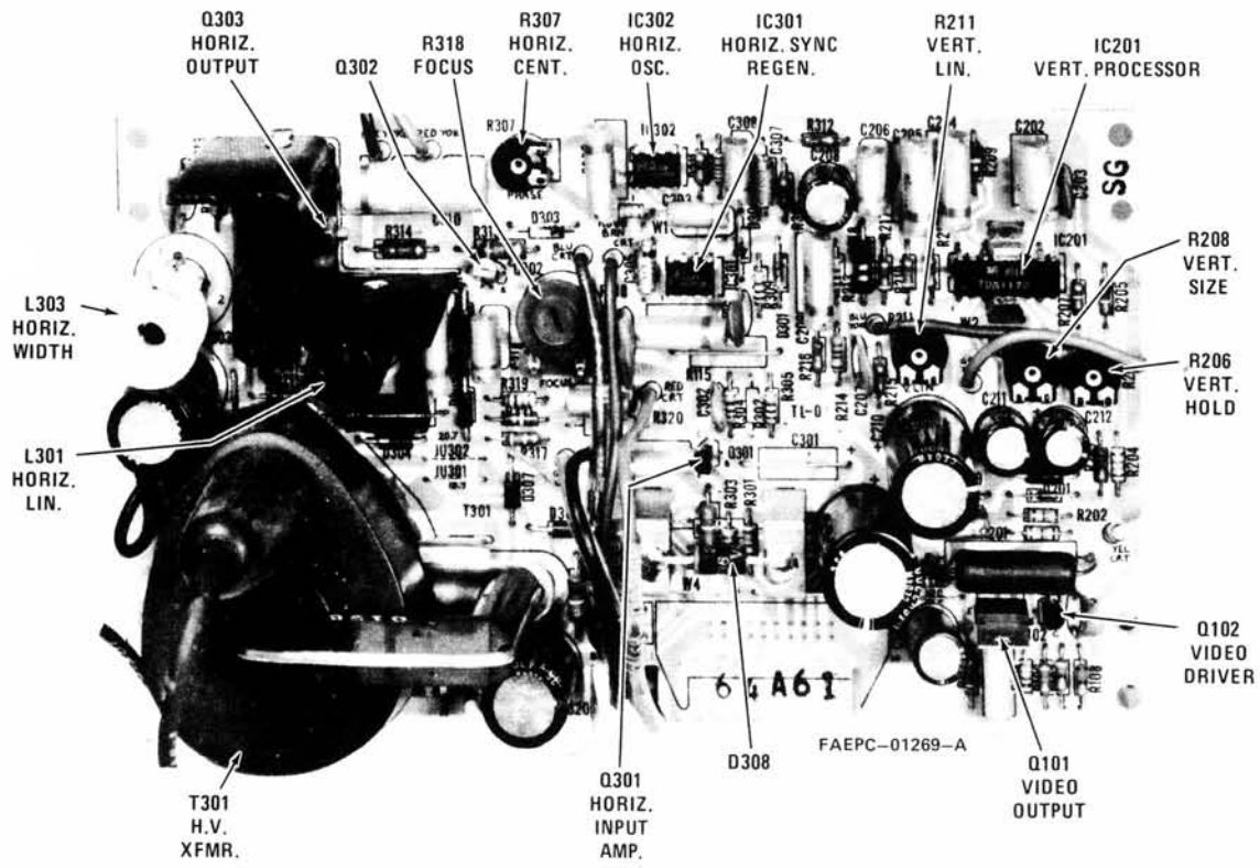
Model MD3570-4/MD3970-4 Series CRT Display Monitor Circuit Card, Component View (Early Version)
