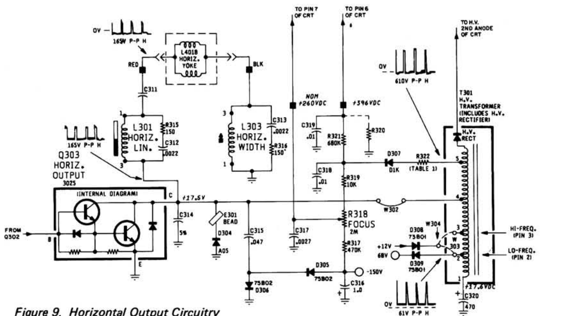
Figure 9. Horizontal Output Circuitry
