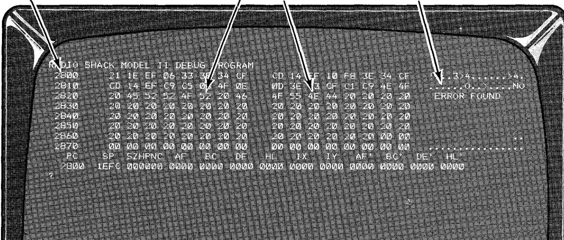
Z-80A register contents. SZHPNC are the flag bits in register F.
