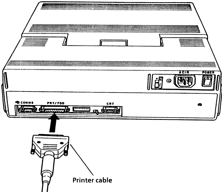
Figure 4-8 Printer Connection
